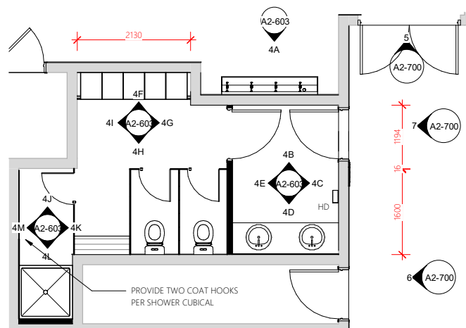
Joinery Plan 4
