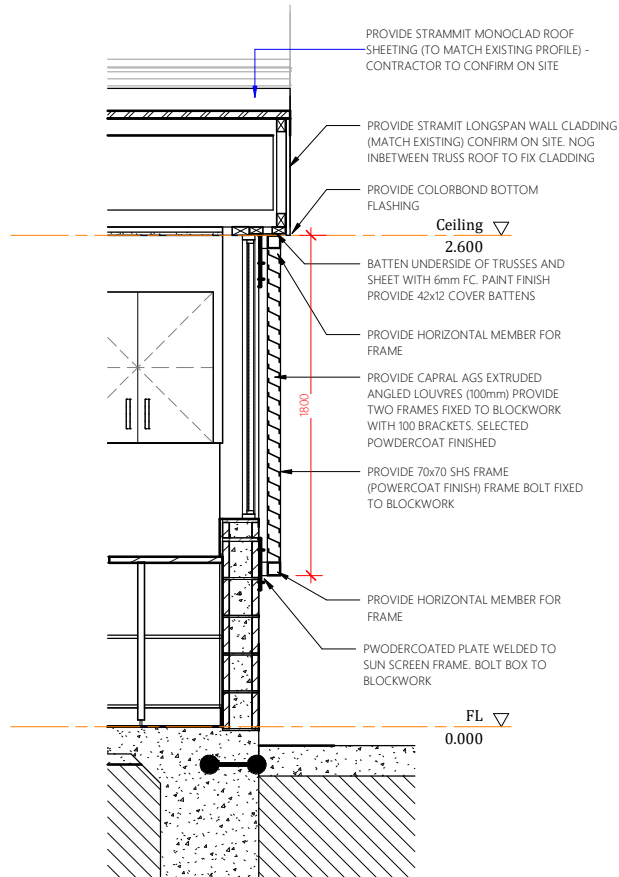
Section B1
