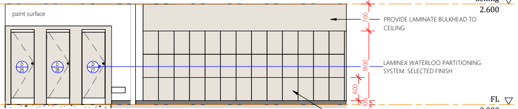
Elevation 5D
