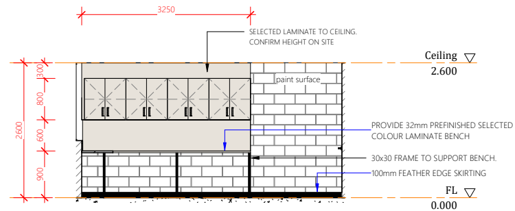
Elevation 1C 1 : 50
